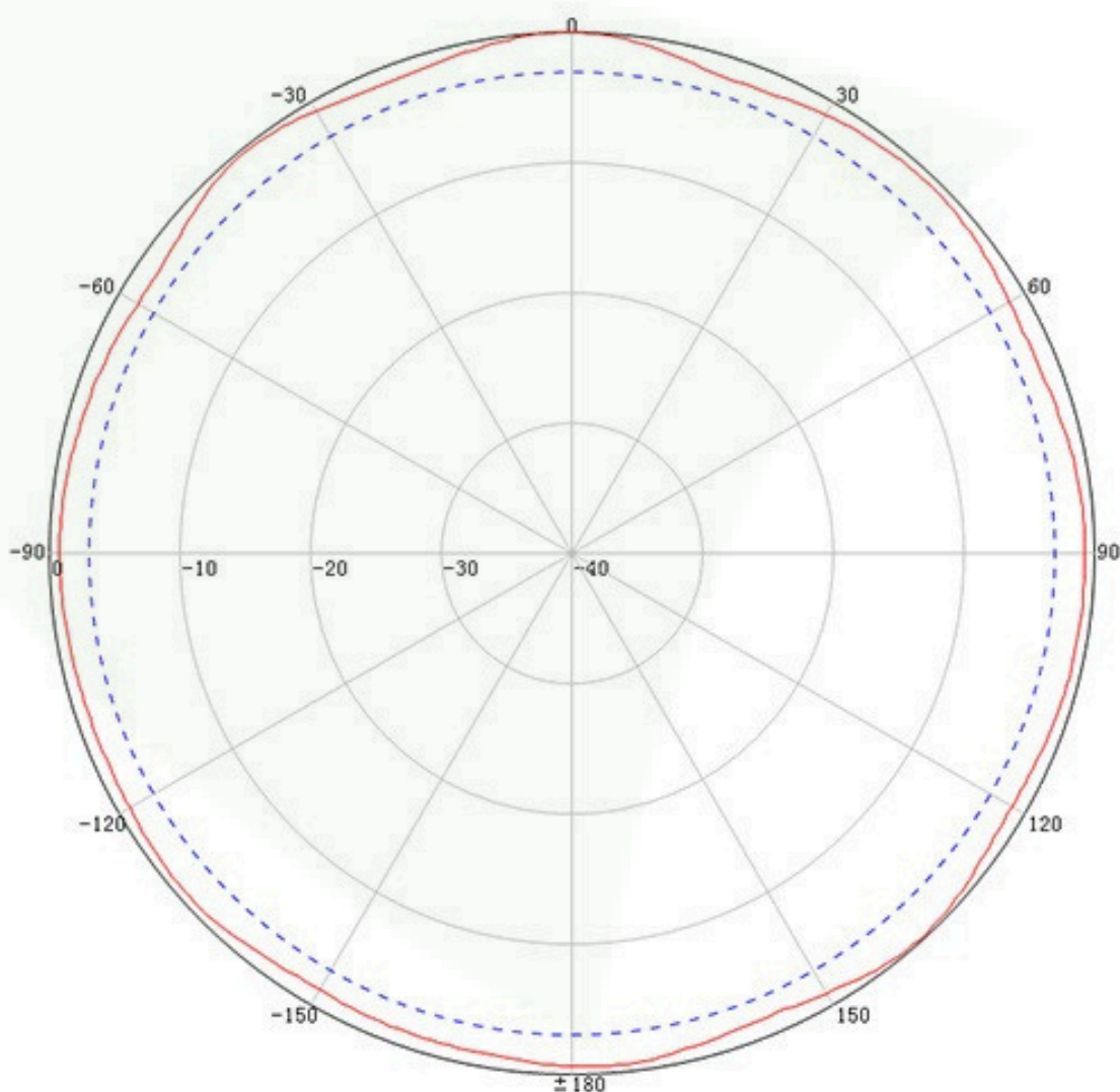
Horizontal Pattern
