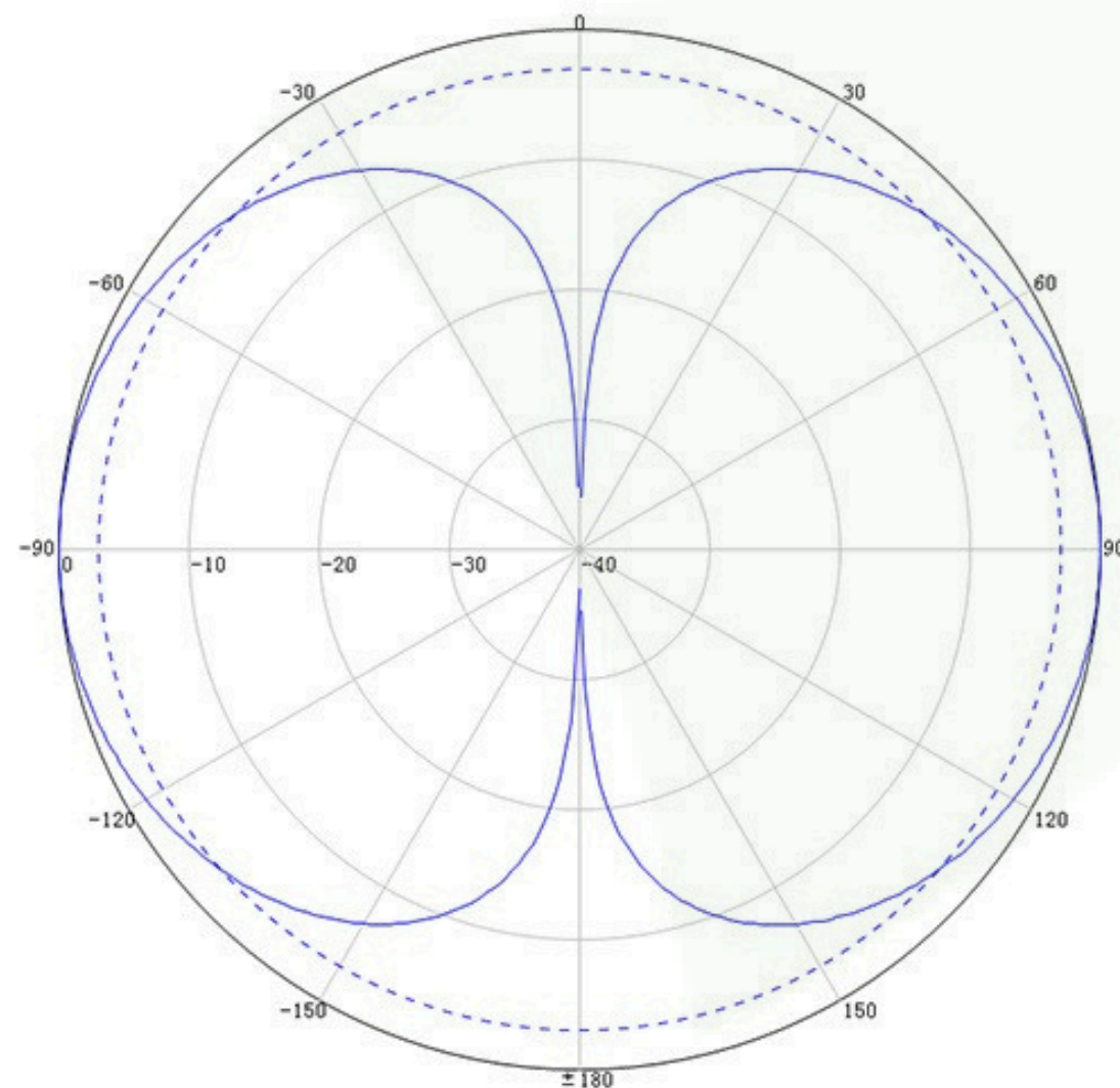
Vertical Pattern
